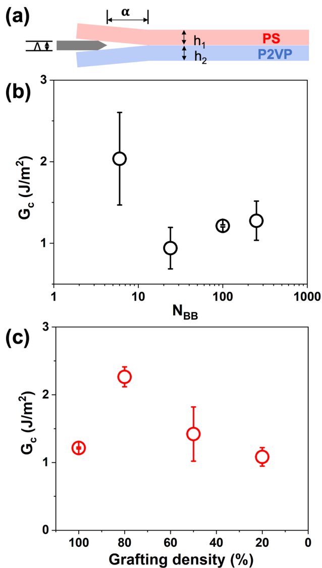
Fig. 9 Adhesion strength of JBCPs at homopolymer interface measured by asymmetric double cantilever beam (ADCBC) test. (a) Scheme of ADCBC test. Critical energy release rate ( G_c ) as a function of (b) N_{BB} (grafting density = 100%) and (c) grafting density ( N_{BB} = 100\% ).
