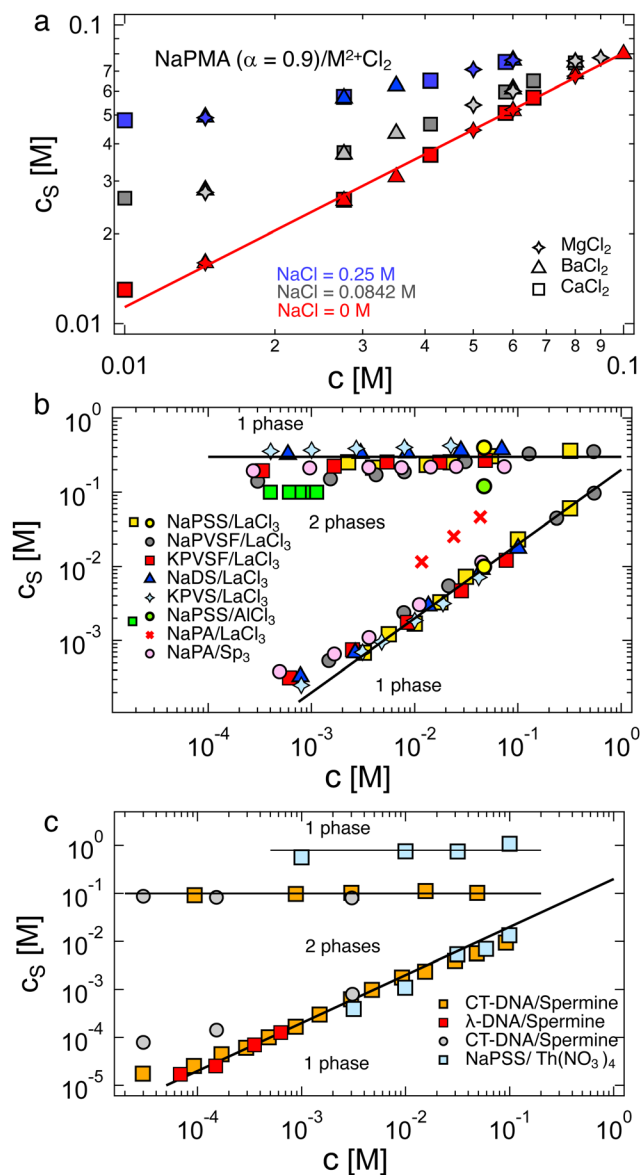
Fig. 5 (a) Added salt concentration as a function of polymer concentration for polymethacrylic acid ( \nu = 0.9 ) in DI water and aqueous NaCl solutions. Line is c_s = 0.57c^{0.85} . Data are from ref. 228. (b) Added salt concentration for precipitation ( c_s^{**} ) and re-dissolution ( c_s^D ) for polyelectrolytes with added trivalent salts. NaPSS/ \text{LaCl}_3 data are from ref. 199 (yellow squares) and ref. 229 (yellow circles), NaPSS/ \text{AlCl}_3 from ref. 202 (green squares) and ref. 229 (green circle) and NaPSS/ \text{LaCl}_3 (red crosses) from ref. 197. Sp stands for trivalent cation spermidine. All others are from ref. 230. Top line is c_s = 0.3M , bottom line is c_s = 0.2c . (c) Precipitation and re-dissolution c_s for DNA and PSS in the presence of tetra-valent ions. NaPSS data are from ref. 199 DNA data are from ref. 231 (squares) and ref. 232 (circles). Bottom line is c_s = 0.2c .
