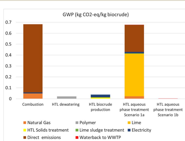
Fig. 7 LCA of HTL biocrude production – contribution of flows and substeps for Scenarios 1a and 1b (total value of the GWP metric is 1.42 CO 2 -eq. per kg biocrude and 0.75 kg CO 2 -eq. per kg biocrude, respectively).
