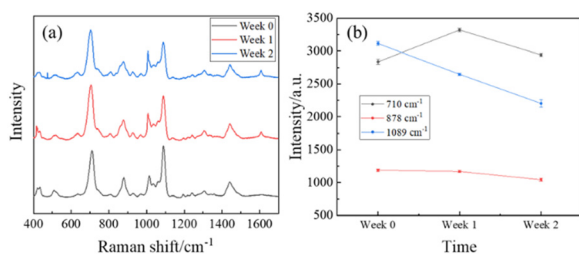
Fig. 8 (a) The time-dependent averaged spectra of 10^6 ppt PFOA on MCH-modified AgNR substrates. Measurements were taken on the day of creation (black, week 0), 1 week after creation (red), and 2 weeks after creation (blue). (b) The intensity of spectra peaks \Delta\nu = 710\text{ cm}^{-1} (black), 878\text{ cm}^{-1} (red), and 1089\text{ cm}^{-1} (blue) versus time.
