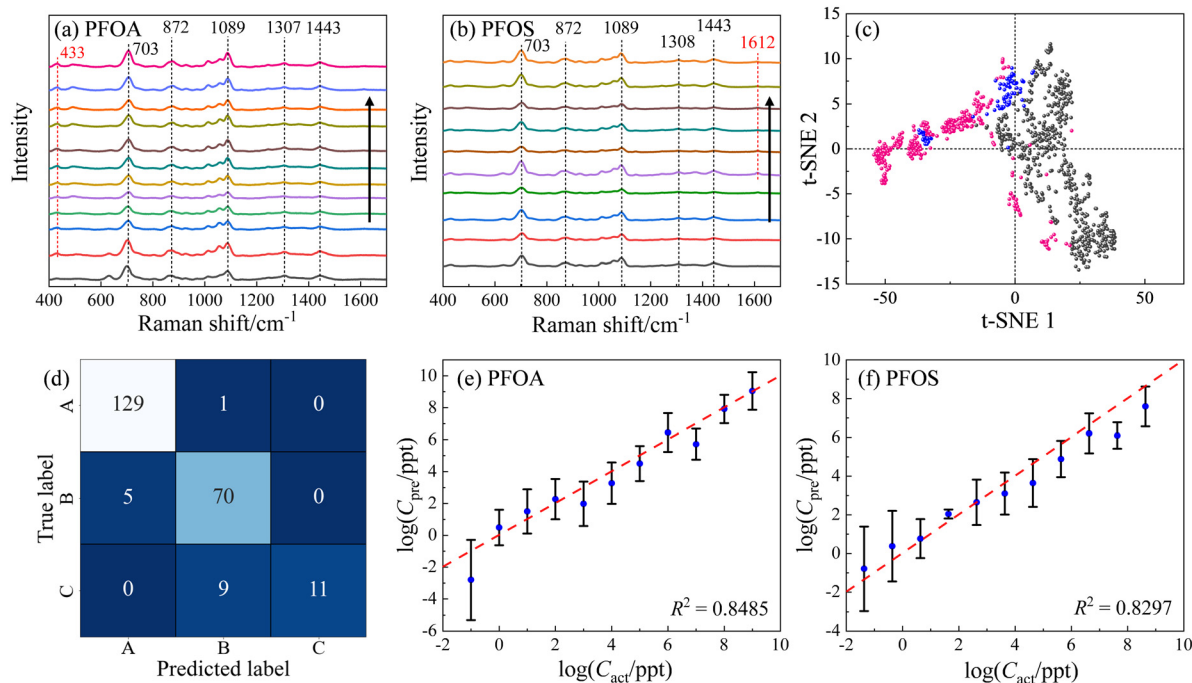
Fig. 6 The average SERS spectra from MCH modified AgNR substrates: (a) PFOA of concentrations of 0, 10^{-1}, 10^0, 10^1, 10^2, 10^3, 10^4, 10^5, 10^6, 10^7, 10^8, and 10^9\text{ ppt} , respectively; and (b) PFOS with concentrations of 0, 4.28 \times 10^{-2}, 4.28 \times 10^{-1}, 4.28, 4.28 \times 10^1, 4.28 \times 10^2, 4.28 \times 10^3, 4.28 \times 10^4, 4.28 \times 10^5, 4.28 \times 10^6\text{ ppt} , respectively. The arrows in the figures indicate the direction of the concentration increase. (c) t -SNE result for PFOS (pink), PFOA (grey), and reference (blue) samples, including spectra from all concentrations. (d) The SVM classification confusion matrix for PFOS, PFOA, and reference samples. A: different concentrations of PFOA; B: different concentrations of PFOS; and C: MCH-modified AgNR substrates. (e) and (f) the log-log plot of C_{pre} versus C_{act} of PFOA and PFOS via two independent SVR models, respectively.
