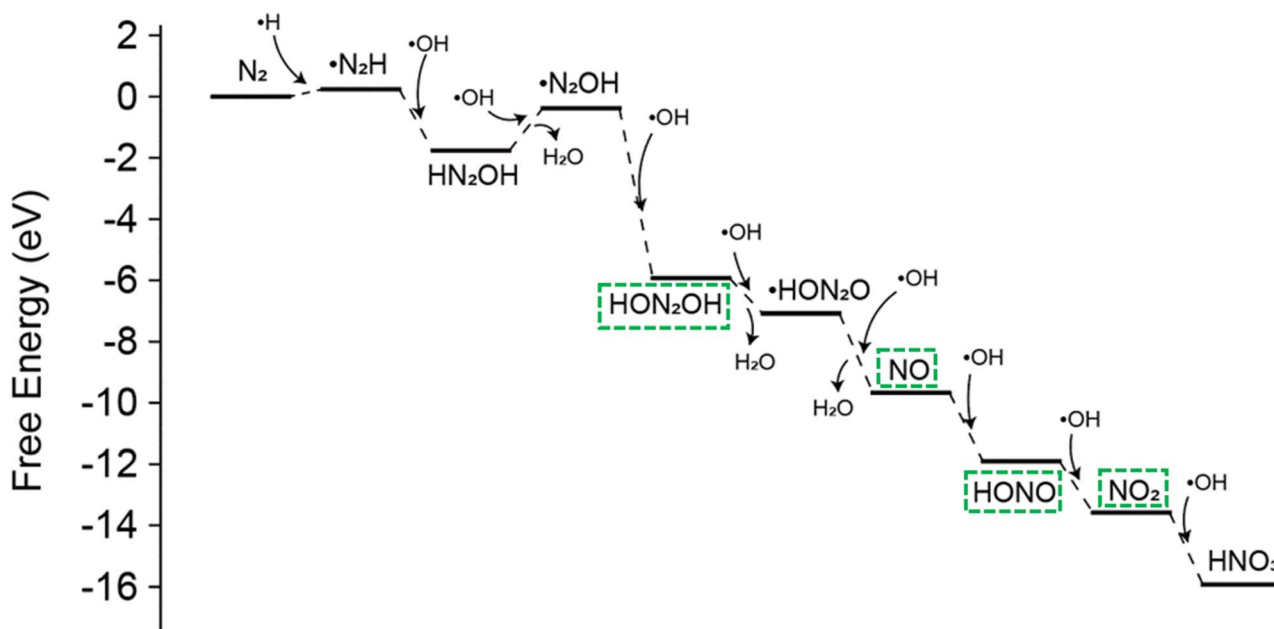
Fig. 5 DFT calculation showing the energy profile of the intermediates involved in the N _2 oxidation to NO _3^- in the microbubbles. The experimentally identified intermediates are shown in green color dashed rectangles.
