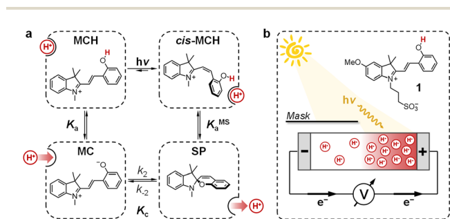
Fig. 2 (a) Four-state model describing MCHs' operation in aqueous environments: visible light-triggered isomerization (upper-right path) contrasts with thermal relaxation (bottom-left path), where the SP ring-opening is the rate-determining step. Substituents are omitted for the sake of clarity. (b) Working principle of the energy harvesting device employed in this study: asymmetric light irradiation of a tube-shaped cell filled with a solution of compound 1 triggers the formation of a persistent proton concentration gradient ( \Delta\text{pH} ) across the cell corresponding to an open circuit voltage, V_{\text{OC}} (mV) = 0.2 \cdot T \cdot \Delta\text{pH} (see below).
