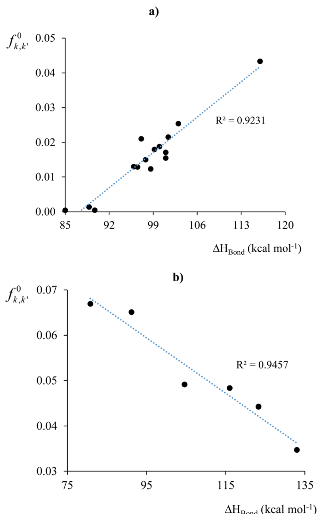
Fig. 4 f_{k,k'}^0 vs. \Delta H_{\text{bond}} profiles for systems with molecular bonds for which (a) \Delta f_{k,k'}^{(2)} < 0 (electron flux destabilized) and (b) \Delta f_{k,k'}^{(2)} > 0 (electron flux stabilized). Figure (a) does not consider the data for the breaking of ethylene to methylene radicals (system 7, ref. 113) due to its large value for f_{k,k'}^0 . Including this reaction would increase the correlation coefficient to 0.967. This figure has been reproduced from ref. 113 with permission from The Royal Society of Chemistry, copyright 2017.
