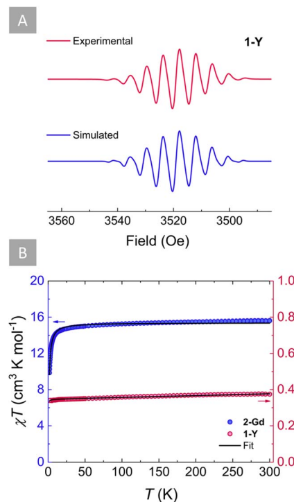
Fig. 4 (A) Experimental (magenta) and simulated (blue) EPR spectra for 1-Y at room temperature and 9.86 GHz (in THF) ( g = 2.0017 ; SW = 20 mT; LW = 0.166 mT; a_N = 0.584 mT). (B) Variable temperature \chi T plots of 1-Y (pink circles) and 2-Gd (blue circles) under an applied static field of 1000 Oe. The solid black lines represent the fits for 1-Y and 2-Gd as determined by applying the -2J formalism.
