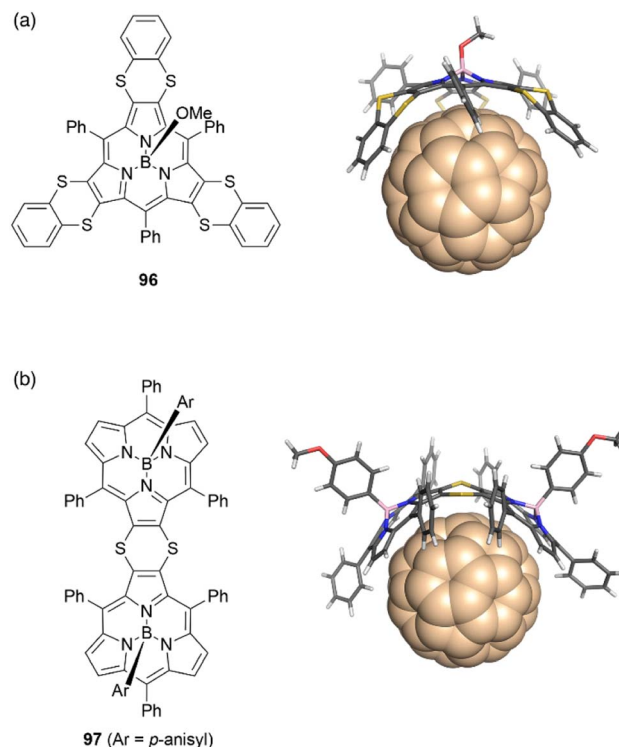
Fig. 10 Crystal structures of fullerene complexes (a) 96 \cdot C_{60} and (b) 97 \cdot C_{60} .
