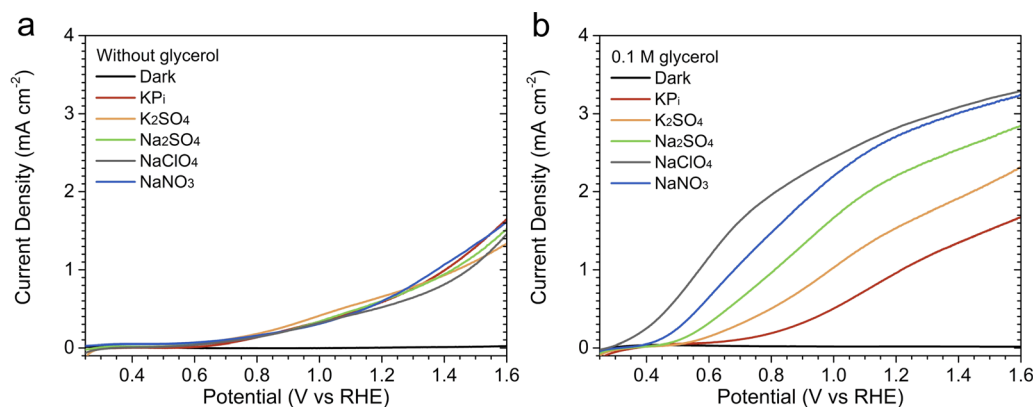
Fig. 1 Linear sweep voltammetry (LSV) curves recorded in different acidic solutions (pH = 2), all having a concentration of 0.5 M: (a) in the absence of glycerol and (b) with 0.1 M glycerol. Measurements were performed at a scan rate of 20 \text{ mV s}^{-1} , sweeping from negative to positive potentials relative to the reversible hydrogen electrode (RHE), under AM 1.5G simulated sunlight illumination. LSV curves recorded in NaNO 3 without illumination are also shown as the representative dark curves; dark LSV curves recorded in other electrolytes are shown in Fig. S3.†
