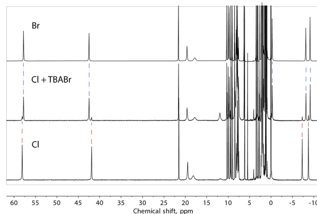
Fig. 8 ^1\text{H} NMR spectra of [\text{Fe}(\text{L}2)_3]^{4+} , from 1 and (\text{Br}@\text{[Fe}(\text{L}2)_3]_2)^{3+} , from 2 , as well as the spectrum obtained by adding one equivalent of TBA bromide to the solution of 1 . Dashed lines are a guide for the eye.
