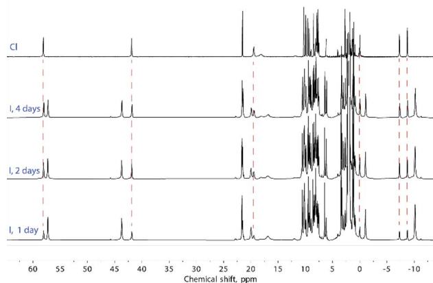
Fig. 6 ^1\text{H} NMR spectra of (\text{I}@\text{[Fe}(\text{L}2)_3]_2)^{3+} , from 3 , and [\text{Fe}(\text{L}2)_3]^{4+} , from 1 . Dashed lines relate the signals that appear from compound ( 3 ) over the course of several days at room temperature with the signals of compound ( 1 ).
