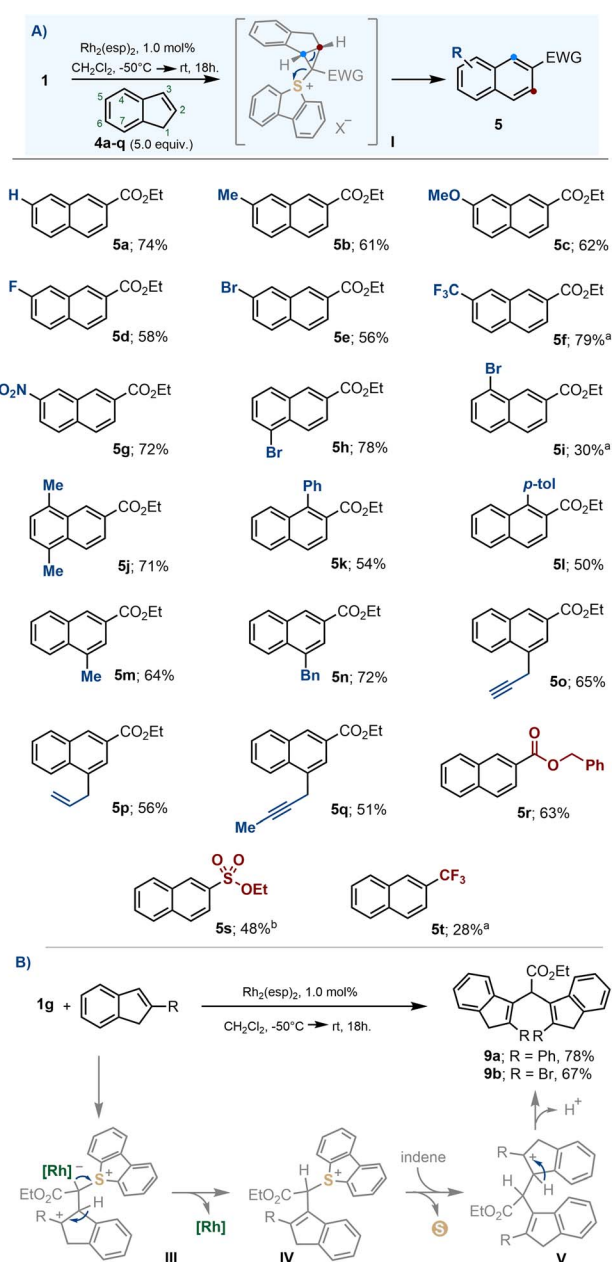
Scheme 5 (A) Substrate scope for the ring expansion from indenones to naphthalenes; (B) dimerization of 2-indenones; a reaction heated at 80 °C for 4 days; b reaction heated at 40 °C for 12 h.
