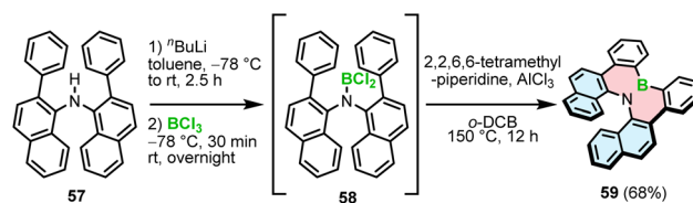
Scheme 11 Synthesis of 1,2-azaborinine helicene 59 .
