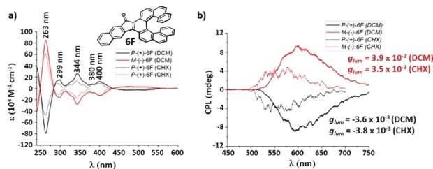
Fig. 8 (a) Circular dichroism spectra of 6F. (b) CPL spectra of (P) and (M) enantiomers of 6F, ( c \approx 1 \times 10^{-5} \text{ M} ).
