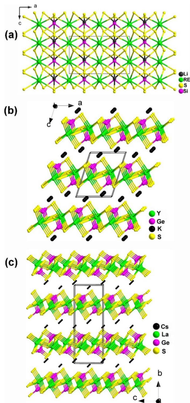
Fig. 11 Structures of (a) LiRESiS 4 (space group: Ama2 ), (b) KYGeS 4 (space group: P2 1 ), and (c) CsLaGeS 4 (space group: P2 1 2 1 2 1 ) with the unit cell outlined.
