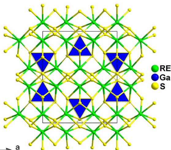
Fig. 1 Structures of RE 3 GaS 6 along the c axis with unit cell and discrete [GaS 4 ] polyhedra (blue) outlined.
