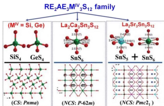
Fig. 10 CS-to-NCS structural transformation with varying anionic motifs in the RE 2 AE 3 M IV 3 S 12 family. This figure has been adapted from ref. 142 with permission from Wiley-VCH, copyright 2024.
