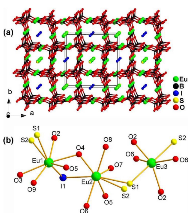
Fig. 22 Structure of (a) \text{Eu}_{4.5}(\text{B}_5\text{O}_9)_2\text{SI} along the ab plane with the unit cell outlined and (b) coordination environment of the crystallographically independent Eu atoms.
