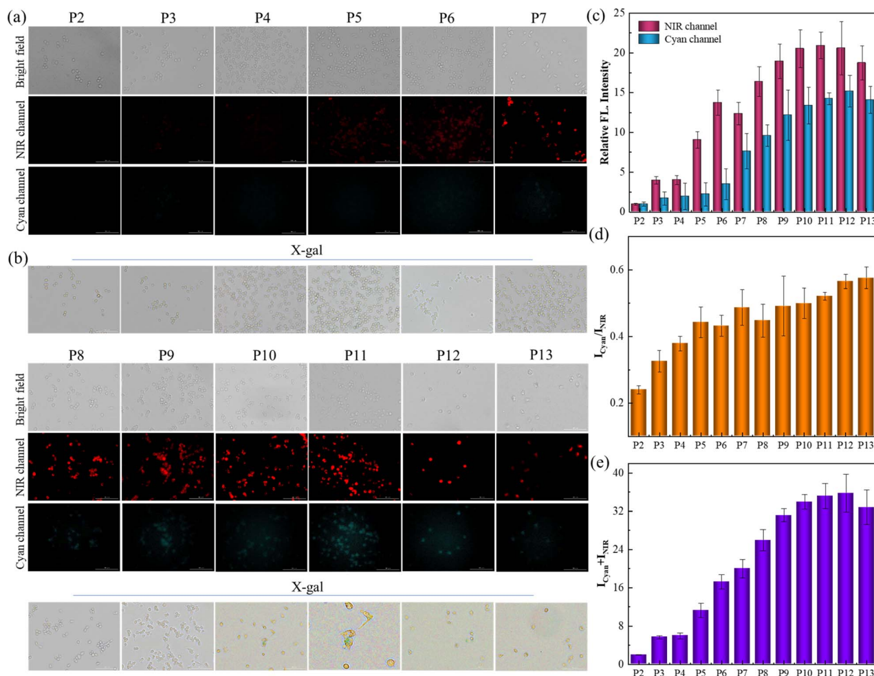
Fig. 5 (a) Fluorescent images of RAW 264.7 cells from P2 to P13 after incubation with 10 μM SA-HCy-1 for 30 min. Top: bright field; middle: NIR channel; ground: cyan channel. For the NIR channel: \lambda_{\text{ex}} = 628 nm, \lambda_{\text{em}} = 670-730 nm; for the cyan channel: \lambda_{\text{ex}} = 377 nm, \lambda_{\text{em}} = 450-500 nm, scale bar = 100 μm. (b) X-gal staining of RAW 264.7 cells from P2 to P13. (c) Quantification of fluorescence intensities of (a) from NIR (red bars) and cyan (blue bars) channels. (d) Quantification of fluorescence intensity ratios ( I_{\text{Cyan}}/I_{\text{NIR}} ) of the images from (a). (e) Quantification of fluorescence intensity sums ( I_{\text{Cyan}} + I_{\text{NIR}} ) of the images from (a). Error bars represent the standard deviation (±S.D.), n = 3.
