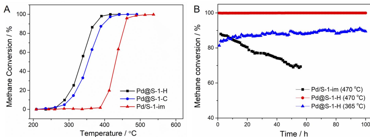
Fig. 3 (A) Catalytic performance of methane combustions over \text{Pd}@\text{S-1-H} , \text{Pd}@\text{S-1-C} , and \text{Pd}/\text{S-1-im} catalysts. Reaction condition: 2% \text{CH}_4 –20% \text{O}_2 –78% \text{N}_2 , gas hourly space velocity (GHSV) = 36\,000\text{ mL g}_{\text{cat}}^{-1}\text{ h}^{-1} . (B) Long-term stability of methane combustions over \text{Pd}@\text{S-1-H} and \text{Pd}/\text{S-1-im} catalysts with a GHSV of 36\,000\text{ mL g}_{\text{cat}}^{-1}\text{ h}^{-1} .
