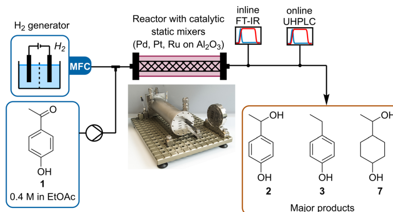
Fig. 1 Schematic representation of the setup used to study the hydrogenation of ketone 1 , using different metal/ \text{Al}_2\text{O}_3 CSMs.
