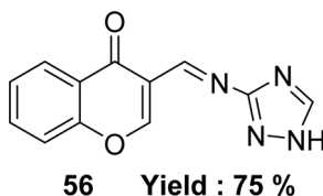
Fig. 33 Structure of Schiff base ligand 56.
