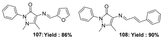
Fig. 48 Structure of Schiff base ligands 97–108.
