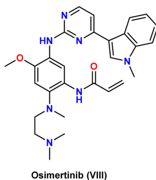
Fig. 2 The chemical structures of reported EGFR-TKIs.
