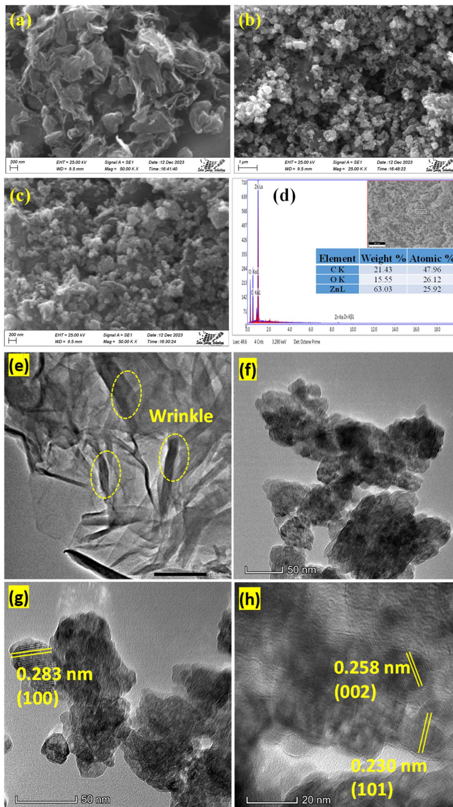
Fig. 1 SEM images of (a) rGO and (b and c) rGO/ZnO. (d) EDX spectrum of rGO/ZnO; TEM images of (e) rGO and (f–h) rGO/ZnO at different magnifications.
