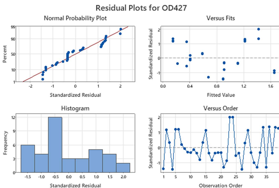
Fig. 1 Residual plots for OD 427 . The plots demonstrate that the data provided for PDB analysis is normally distributed without outliers.
