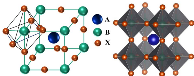
Fig. 6 The basic structure of ABX_3 with corner-sharing BX_6 octahedral.
