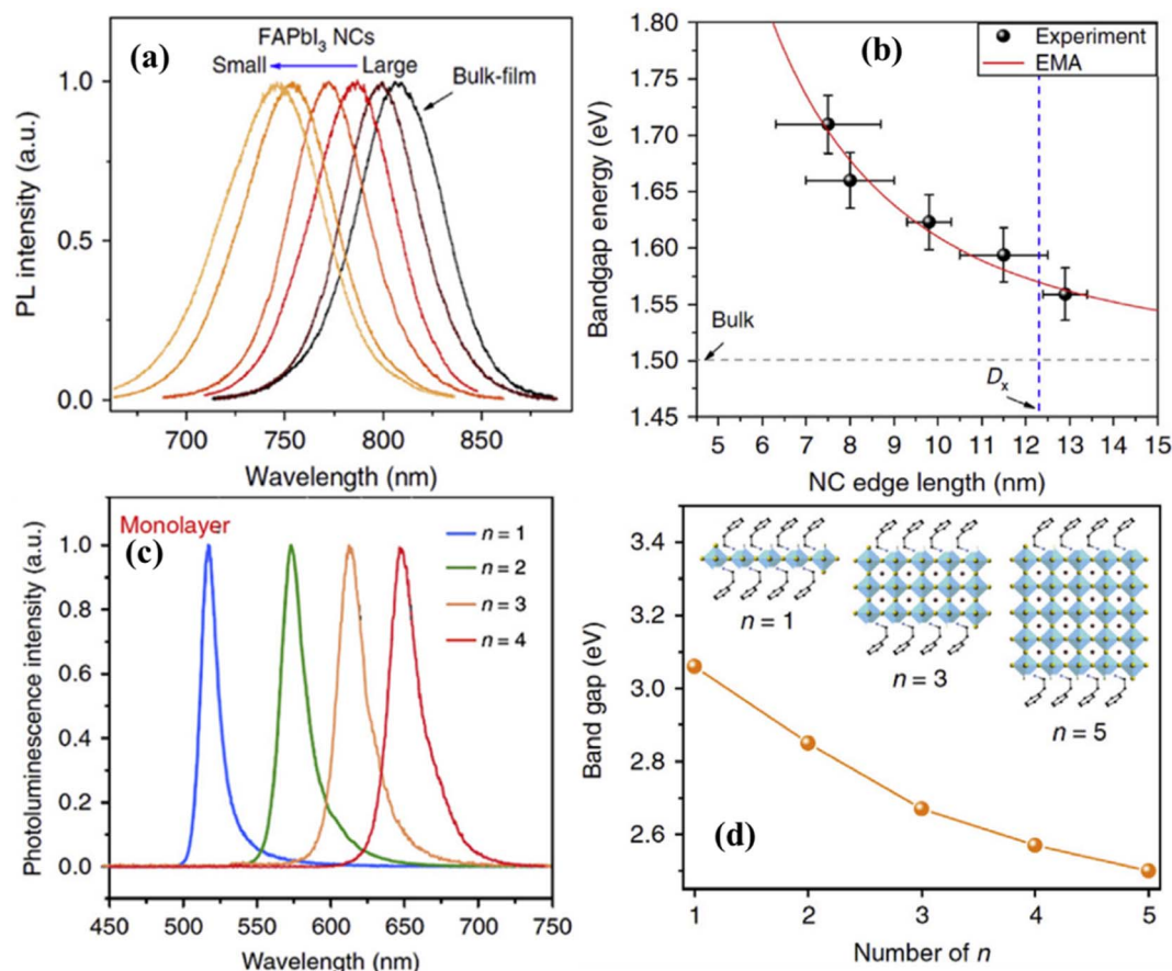
Fig. 17 Bandgap engineering by modifying the dimensionality. (a) Size-dependent PL spectra of \text{FAPbI}_3 NCs. (b) Bandgap versus edge length of \text{FAPbI}_3 NCs. Reproduced from ref. 175 with permission from Springer Nature, copyright 2018. (c) PL spectra of exfoliated monolayers for 2D \text{BA}_2(\text{MA})_{n-1}\text{PbI}_{3n+1} Ruddlesden-Popper perovskites of n = 1 to 4 homologues. Reproduced from ref. 187 with permission from Springer Nature, copyright 2018. (d) The bandgap of \text{PEA}_2\text{A}_{1.5}\text{Pb}_{2.5}\text{Br}_{8.5} ( \text{A} = \text{MA} and \text{Cs} ) perovskites with different numbers of layers. Reproduced from ref. 44 with permission from Springer Nature, copyright 2018.
