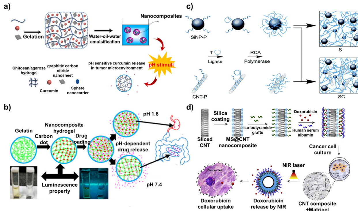
Fig. 4 Mechanism of drug delivery based on carbon-based nanocomposites. (a) Schematic diagram of a pH-sensitive nanocarrier composed of chitosan, agarose, graphitic carbon nitride, and curcumin. Reproduced from ref. 79 with permission from Elsevier, copyright 2022, (b) scheme of carbon dot-gelatin nanocomposite hydrogel for delivery of cefadroxil. Reproduced from ref. 80 with permission from American Chemical Society, copyright 2020, (c) schematic illustration of programmable drug delivery system based on silica nanoparticle/CNT-DNA nanocomposites. Reproduced from ref. 81 with permission under the terms of the CC-BY Creative Commons attribution 4.0, and (d) schematic diagram of a mesoporous silica (MS)-modified CNT nano-platform. Reproduced from ref. 82 with permission from Elsevier, copyright 2020.
