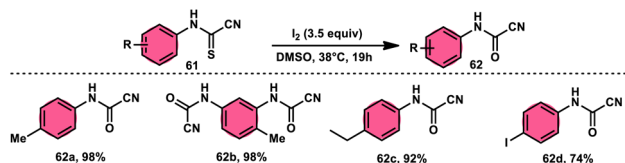
Scheme 35 Synthesis of N -arylcyanoformamide 62 and representative examples.
