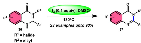
Scheme 21 Intramolecular oxidative cross-coupling reaction mediated by \text{I}_2/\text{DMSO} .
