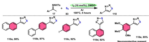
Scheme 67 Synthesis of thiadiazoles 110 using I 2 /DMSO system.
