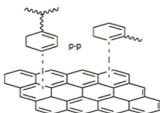
Fig. 20 Crystalline graphite powder with an aqueous solution of PVP under sonication which resulted in water-soluble polymer-protected graphene single layer. (a) CH- \pi bonding under polyethylene (PE), polyvinylpyrrolidone (PVP) polyvinylchloride (PVC), cellulose, chitosan and pullulan treatment, (b) \pi - \pi stacking (under poly(3,4-ethylenedioxythiophene) (PSS), polyhexahydrotriazine (PHT), lignin, dye-polyvinyl alcohol (dye-PVA), cytosine-polypropylene glycol (cytosine-PPG) and pyrene-polyethylene (pyrene-PE) treatment and (c) cation- \pi interaction.
