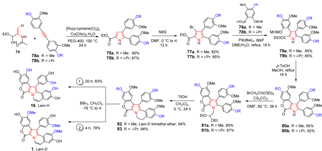
Scheme 4 Total synthesis of lam-D (1), lam-H (16), and lam-D trimethyl ether (82), through various \text{Ru}(\text{II}) -catalyzed C-H activations.
