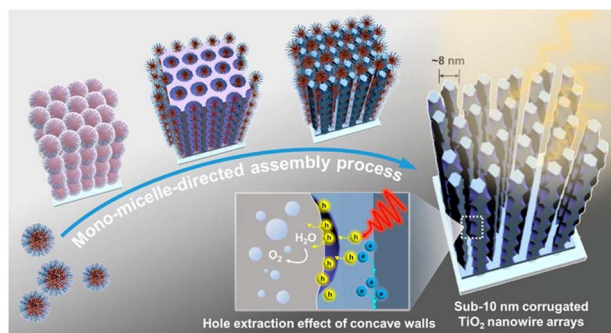
Fig. 7 Schematic illustration of the formation process for the ultrathin corrugated TiO 2 nanowire arrays synthesized via the monomicelle-directed assembly approach. 142
