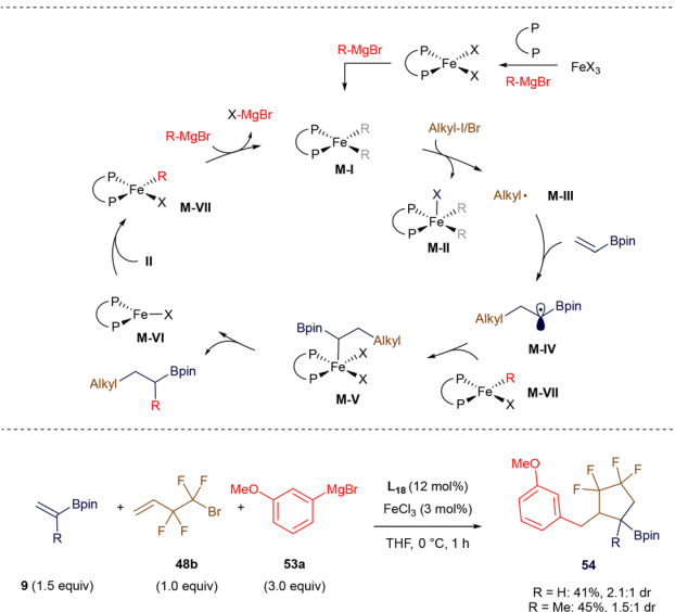
Scheme 19 Iron-catalyzed 1,2-biscarbofunctionalization.
