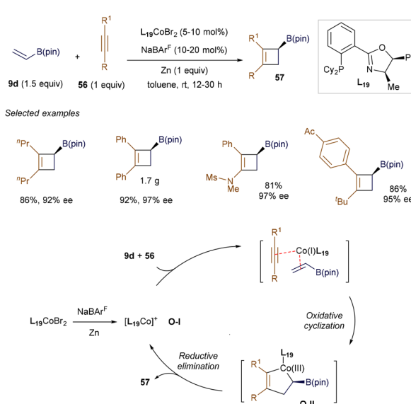
Scheme 21 Co(I)-catalyzed [2 + 2] cycloaddition.
