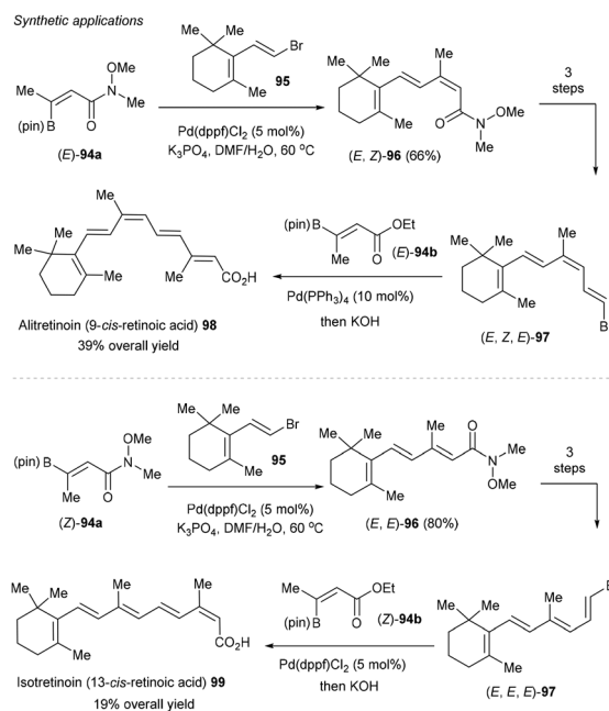
Scheme 37 Synthetic applications.
