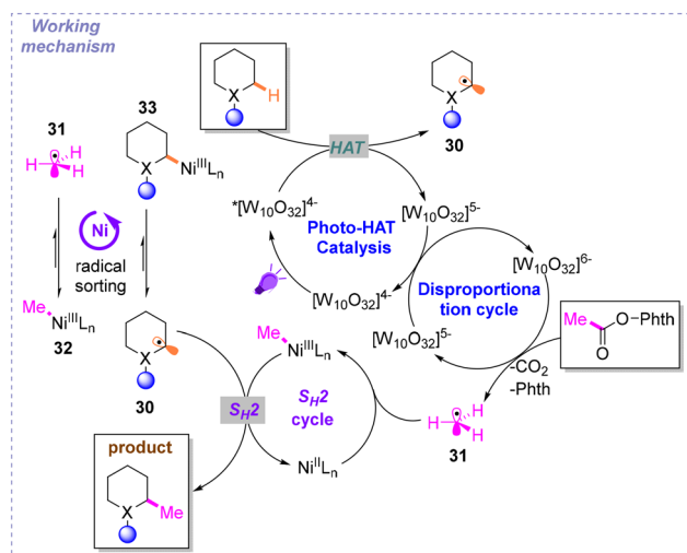
Scheme 12 Methylation of saturated heterocyclic Csp 3 -H bonds.
