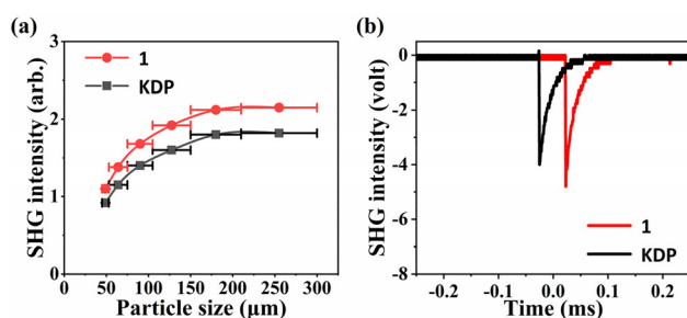
Fig. 5 (a) SHG intensity vs. particle sizes at \lambda = 1064 nm for 1 . (b) SHG signals of 1 as compared with the KDP reference.
