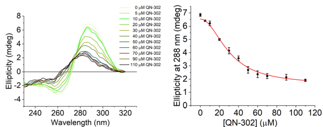
Fig. 4 Left: CD titration of the C-rich S100P sequence (10 \mu M) and QN-302 (0–110 \mu M) in 10 mM lithium cacodylate and 100 mM KCl buffer at pH 5.5. Right: plot of ellipticity at 288 nm against QN-302 concentration and corresponding Hill 1 fitting.
