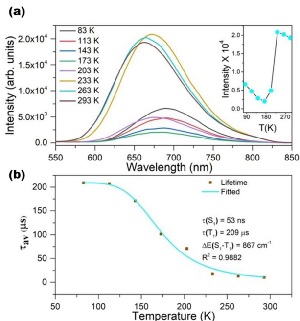
Fig. 4 (a) Temperature-dependent emission spectra of Ag 22 nano-clusters at 365 nm excitation. Inset: temperature-dependent solid-state photoluminescence intensity from 83 to 293 K. (b) Plot of photoluminescence lifetime at 670 nm against temperature for Ag 22 and the data fitting. Reproduced from ref. 114 with permission from Wiley, copyright (2022).
