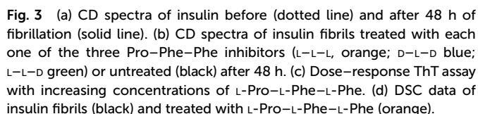
equivalent of Pro-Phe-Phe relative to insulin, which in the case of the test corresponded to 14 \mu M. An excess of inhibitor led to a maximum reduction of fibrillation by approximately 75%, in agreement with the ThT data shown in Fig. 1.
