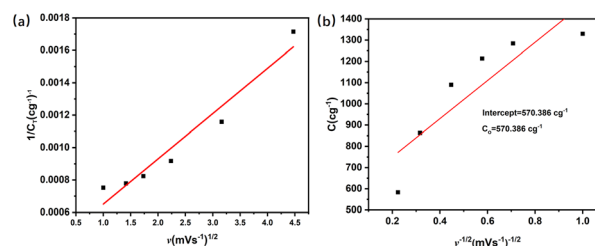
Fig. 9 Kinetic characteristics and reaction mechanism of CoNi 0.5 -MOF/CC electrode: (a) fitting theoretical capacity; (b) fitting theoretical capacitive capacity (Trassatti's method).
