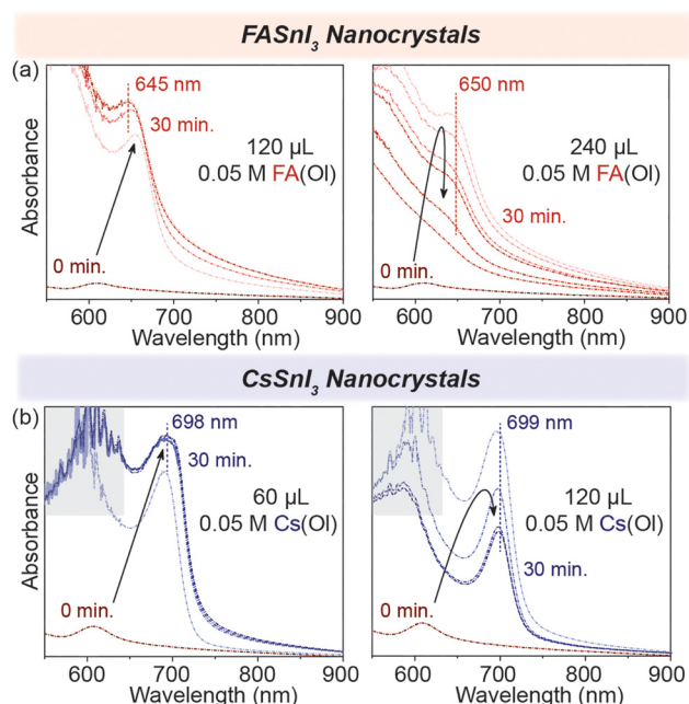
Fig. 3 Concentration dependence in situ UV-visible absorption spectroscopy. (a) The formation of the 3D FASnI 3 (red) NCs with the addition of FA(OI) in the 2D [R-NH 3 ] 2 SnI 4 RP structures for 30 min. (b) The formation of the 3D CsSnI 3 (blue) NCs with the addition of Cs(OI) in the 2D [R-NH 3 ] 2 SnI 4 RP structures for 30 min. The grey area highlights the detector saturation region in the above plots.
