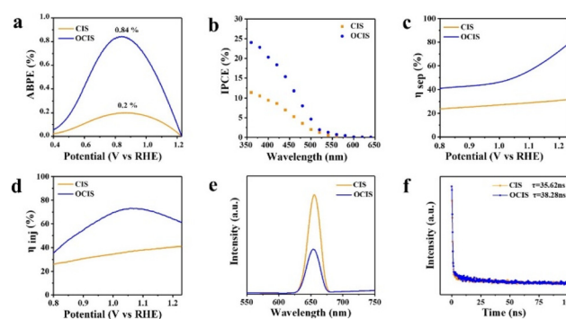
Fig. 4 (a) ABPE and (b) IPCE for CIS and OCIS. (c) Charge separation efficiency and (d) charge injection efficiency of CIS and OCIS. (e) Steady-state PL spectra for CIS and OCIS with excitation wavelength \lambda_{ex} = 325 \text{ nm} . (f) TRPL decay spectra for CIS and OCIS.
