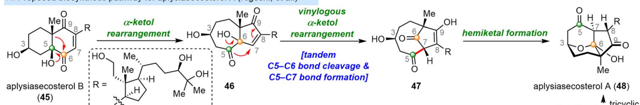
B. Bioinspired synthetic design of the tricyclic cage skeleton (Gui, et al.)
