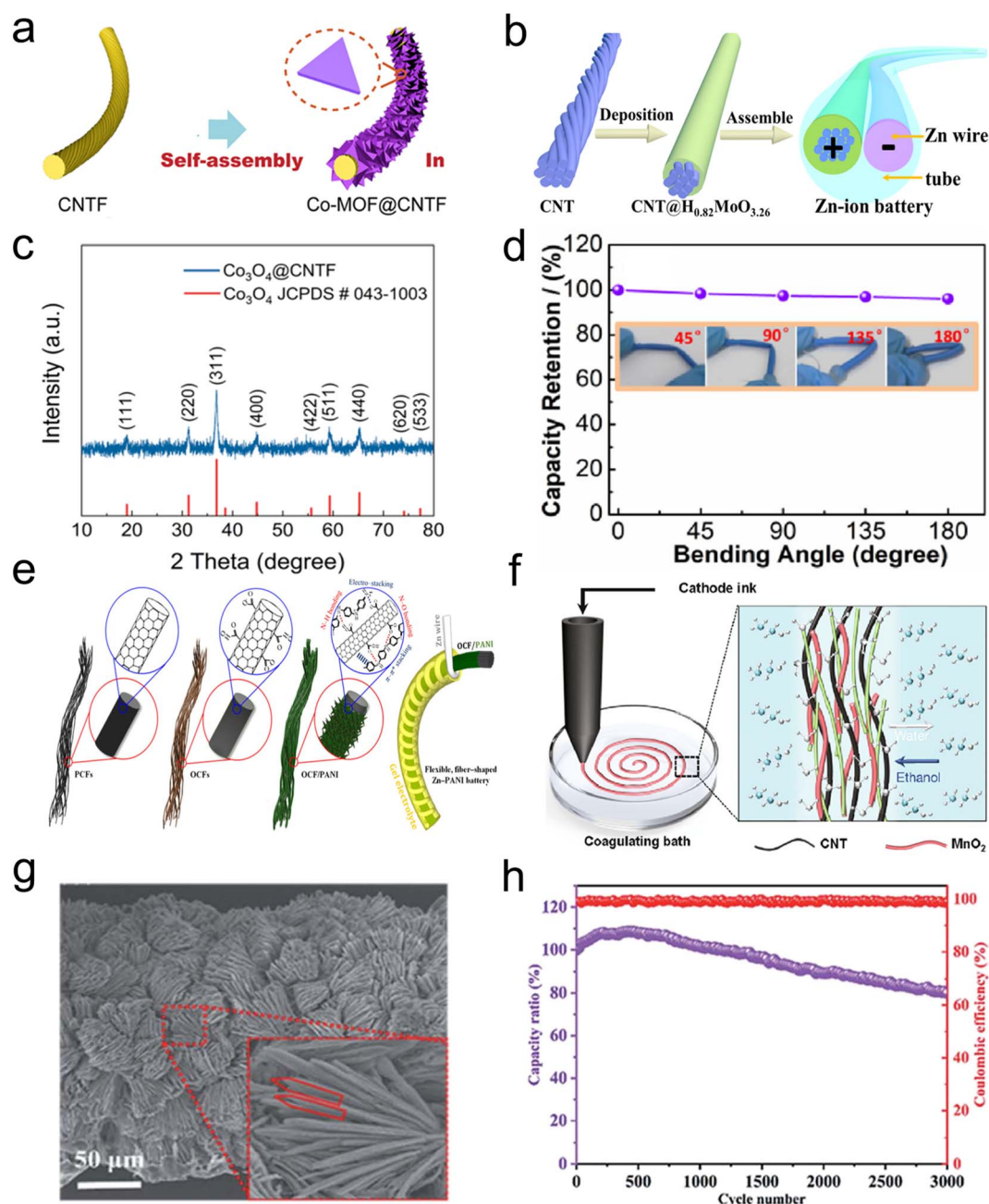
Fig. 4 (a) Schematic diagram of the preparation process of fiber-shaped \text{Co}_3\text{O}_4@CNT electrodes and (c) XRD pattern of the \text{Co}_3\text{O}_4@CNT s. Reproduced with permission from ref. 44. Copyright 2021 American Chemical Society. (b) Schematic illustration of the fiber-shaped Zn-ion battery and (d) the capacity retention at different bending angles. Reproduced with permission from ref. 77. Copyright 2022 Elsevier. (e) Schematic preparation of OCF/PANI electrode-based flexible FZIBs. Reproduced with permission from ref. 88. Copyright 2020 American Chemical Society. (f) Wet-spun fiber-shaped electrodes. Reproduced with permission from ref. 37. Copyright 2022 Elsevier. (g) SEM image of the \text{Mn}_2\text{O}_3@C/CNT electrode and (h) cycling performance of the FZIBs at 3 \text{ A cm}^{-3} . Reproduced with permission from ref. 96. Copyright 2020 Royal Society of Chemistry.
