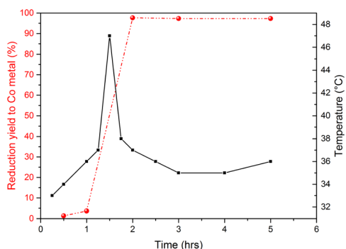
Fig. 6 Co conversion and bowl temperature as functions of milling time. Milling conditions: 7 balls of 10 mm diameter, 3 g of powder (Al + LCO), milling/rest cycle = 15 min/10 min, P/B = 0.15, and n_{\text{Al}}/n_{\text{LCO}} = 1.0 .
