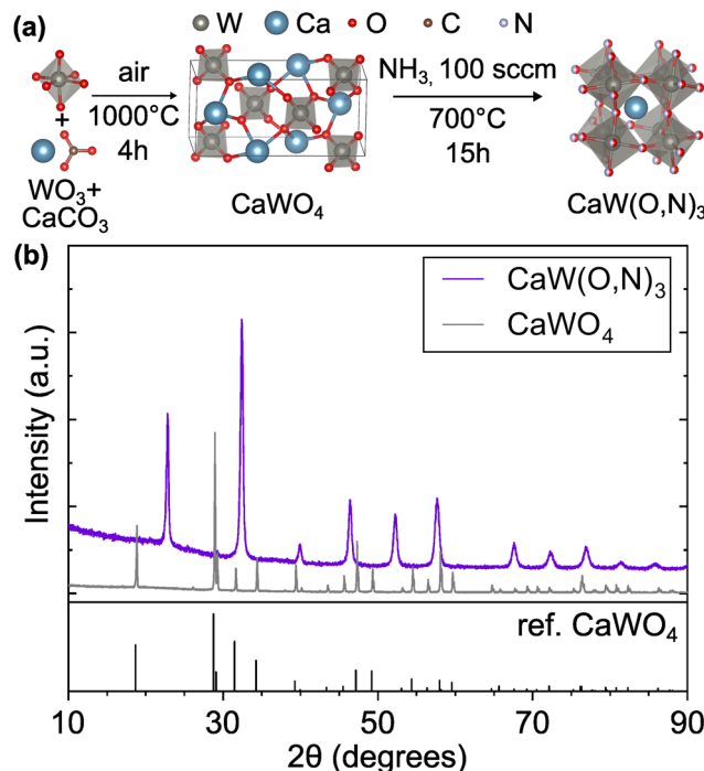
Fig. 1 (a) Synthesis route for CaW(O,N) 3 consisting of calcination of WO 3 and CaCO 3 precursors followed by ammonolysis of the scheelite CaWO 4 intermediate. (b) XRD patterns of intermediate scheelite phases, CaWO 4 and CaW(O,N) 3 , demonstrating their differing crystal structures. CaWO 4 reference is provided. 29 Crystal structure images generated using VESTA. 50
