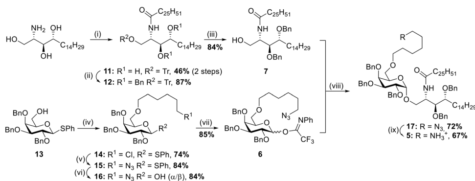
Scheme 1 (i) a. Hexacosanoic acid-NHS ester, \text{Et}_3\text{N} , THF, 50 °C, o/n. b. \text{TrCl} , pyridine, DMAP, 80 °C, o/n; (ii) \text{BnBr} , NaH (60% dispersion in mineral oil), TBAI, anhydr. DMF, 0 °C to RT, 2 h; (iii) p\text{-TsOH} , MeOH, 3 h; (iv) 6-chlorohexyl 4-methylbenzenesulfonate, NaH (60% dispersion in mineral oil), anhydr. DMF, 0 °C to RT, 3.5 h; (v) \text{NaN}_3 , DMF, 80 °C, o/n; (vi) NBS, acetone/H 2 O, 0 °C, 1 h; (vii) 2,2,2-trifluoro-N-phenylacetimidoyl chloride, \text{Cs}_2\text{CO}_3 , anhydr. \text{CH}_2\text{Cl}_2 , RT; (viii) TMSOTf, anhydr. THF/Et 2 O, -20 °C, 1 h; (ix) Zn, AcOH, \text{CH}_2\text{Cl}_2 , RT, 45 min.
