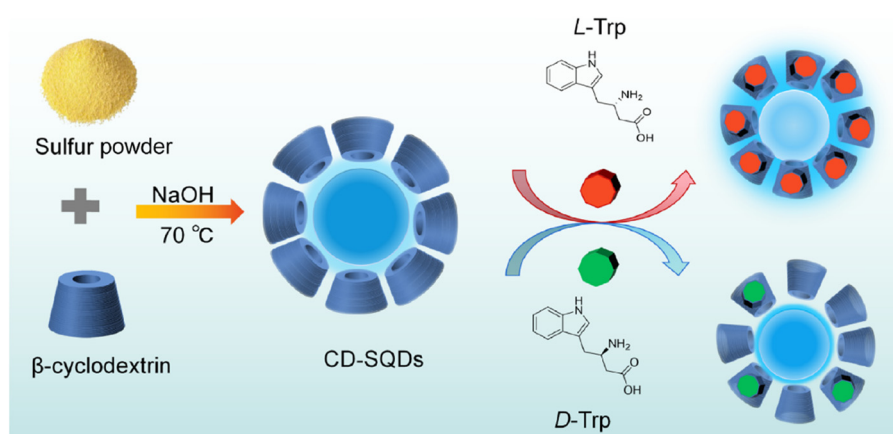
Fig. 12 Schematic illustration of the sensing of L and D-Trp. From ref. 132 with permission. Copyright 2023, American Chemical Society.
