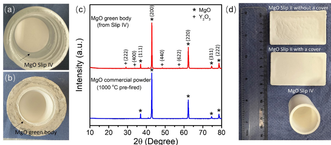
Fig. 7 Assessment and characterisation of slip IV. (a) Photograph of MgO slip IV (water-based). (b) photograph of the MgO green body drying in mould derived from slip IV (size: 35.4 mm in diameter and 41.2 mm in height). (c) XRD patterns of 1000 °C pre-fired MgO powder and the MgO green body originating from slip IV. XRD diffraction peaks corresponding to MgO and Y_2O_3 are referenced to PDF No. 45-0946 and 43-1036. (d) Final MgO products after sintering at 1610 °C derived from slip II and slip IV.
