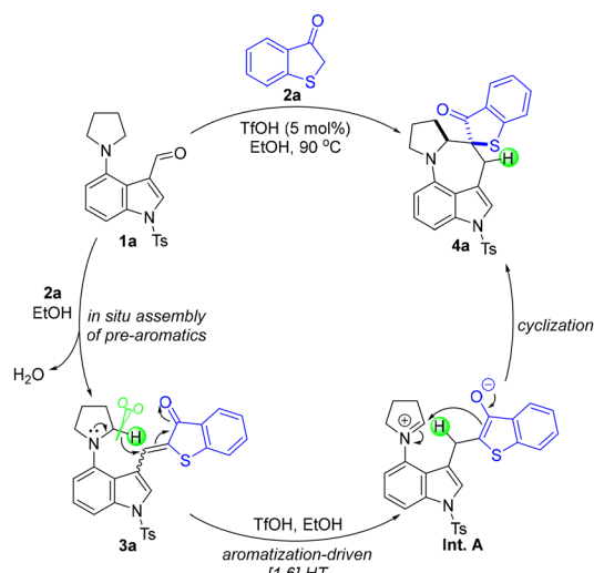
Scheme 6 Proposed mechanism.
