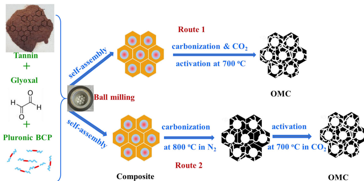
Fig. 14 Diagrammatic representation of the two processes used in the mechanochemical synthesis of OMCs: carbonization under \text{N}_2 and subsequent \text{CO}_2 activation (route 2); one-step carbonization and \text{CO}_2 activation (route 1) utilizing tannin, glyoxal, and block copolymer 327 [reproduced from ref. 327; open access article, copyright permission is not required].
