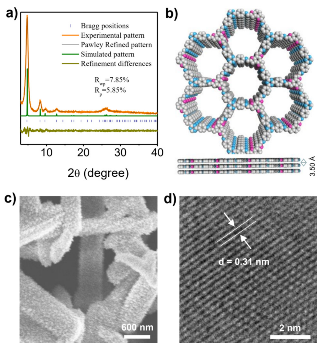
Fig. 4 (a) Experimental and simulated powder X-ray diffraction patterns of COF-JLU42. (b) Top and side views of the AA stacking structure of COF-JLU42 (gray, C; light blue, N; pink, S; O; H atoms are omitted). (c) FE-SEM image of COF-JLU42. (d) HR-TEM image of COF-JLU42.
