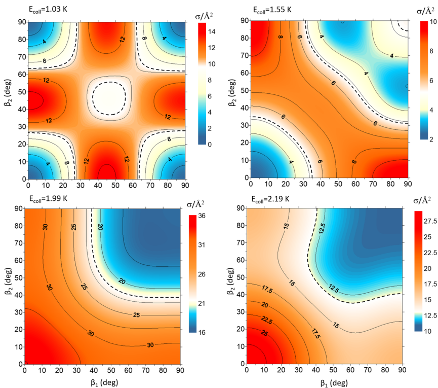
Fig. 9 Contour maps showing the \sigma^{\beta_1\beta_2} for \text{D}_2(v=2, j=2) + \text{D}_2(v=2, j=2) \rightarrow \text{D}_2(v=2, j=2) + \text{D}_2(v=2, j=0) collisions as a function of \beta_1 and \beta_2 for each of the four E_{\text{coll}} highlighted in Fig. 7. Since both \text{D}_2 molecules are indistinguishable \beta_1 and \beta_2 represent the angles that define the direction of the internuclear axis of any of the two diatoms.
