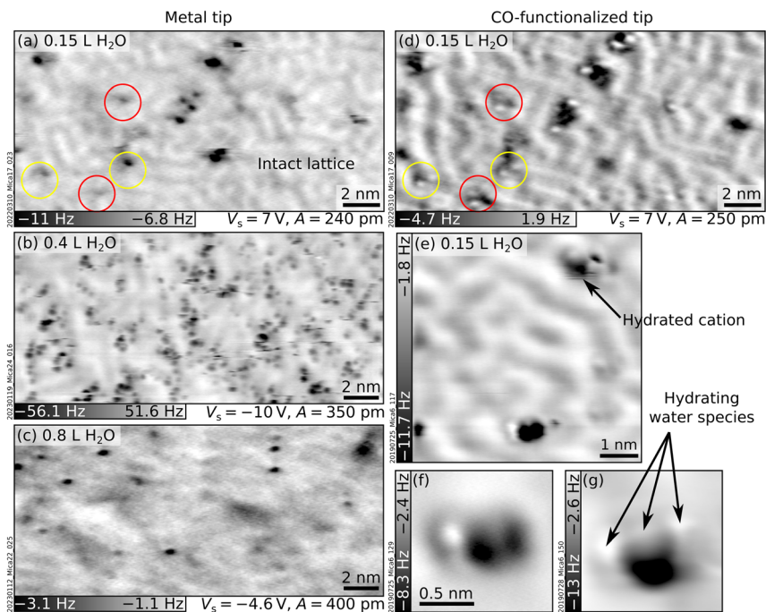
Fig. 2 Mica after exposure to water vapor at 100 K. AFM images acquired at T = 4.7 K with metallic (left) and CO-functionalized (right) tips of UHV-cleaved mica plus sub-monolayer amounts of water vapor dosed at 100 K (doses expressed in Langmuir, L). (a and d) 20 \times 9.8 nm 2 images of the same area after dosing with 0.15 L H 2 O. Circles highlight the most representative protruding features. (b and c) 20 \times 9.3 nm 2 images after 0.4 L and 0.8 L H 2 O, respectively. (e–g) Examples of hydrated cations: (e) 6 \times 6 nm 2 , (f and g) 1.5 \times 1.5 nm 2 , A = 50 pm, V_s = 8 V.
