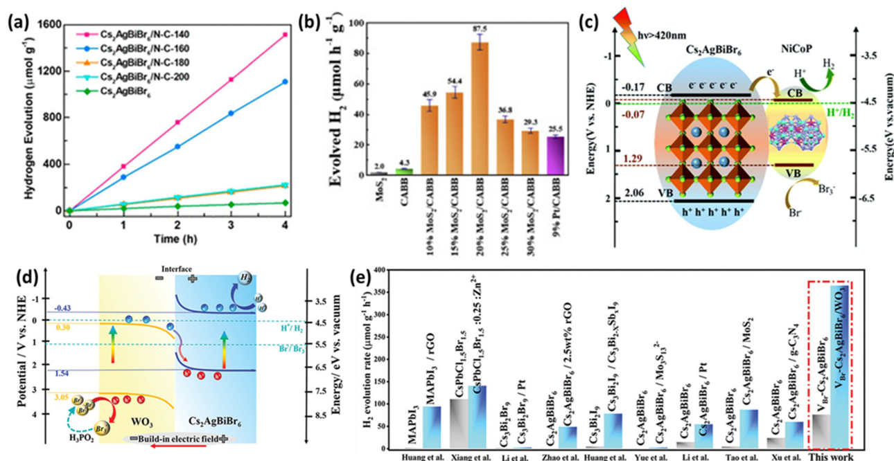
Fig. 6 (a) Hydrogen production rate from HBr aqueous solution using Cs_2AgBiBr_6 and Cs_2AgBiBr_6 /N-C-Th composites under visible light with a cutoff filter ( \lambda \geq 420 nm ), and stability assessment. 91 Reproduced with permission from ref. 91 Copyright © 2021, American Chemistry Society. (b) Photocatalytic hydrogen evolution rates for MoS_2 , CABB, MoS_2/CABB , and Pt/CABB under visible light illumination ( 300 mW cm^{-2} , \lambda \geq 420 nm ). 93 Reproduced with permission from ref. 93 Copyright © 2021, American Chemical Society. (c) Mechanism for photocatalytic hydrogen generation over NiCoP (NCP)/ Cs_2AgBiBr_6 (CABB). 94 Reproduced with permission from ref. 94 Copyright © 2022 Royal Society of Chemistry. (d) Schematic representation of charge transfer and dynamic equilibrium processes. (e) Comparative analysis of hydrogen evolution performance between previously reported perovskite-based catalysts and VBr-Cs_2AgBiBr_6/WO_3 . 98 Reproduced with permission from ref. 98 Copyright © 2023 Wiley-VCH GmbH.
